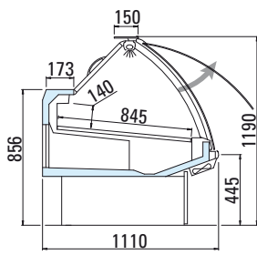
VCA riserva/storage
