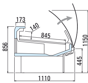
VCB riserva/storage
