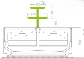
WNE/WDE - 01/03/04/06/07 - TWO LEVELS SUPERSTRUCTURE
