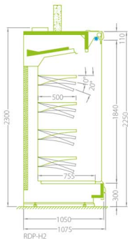
BACK-LOADED EQUIPMENT
