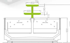
WNE/WDE - 01/03/04/06/07 - TWO LEVELS SUPERSTRUCTURE
